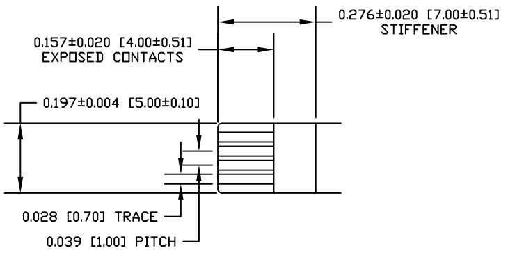
DETAIL A SCALE 4.0
